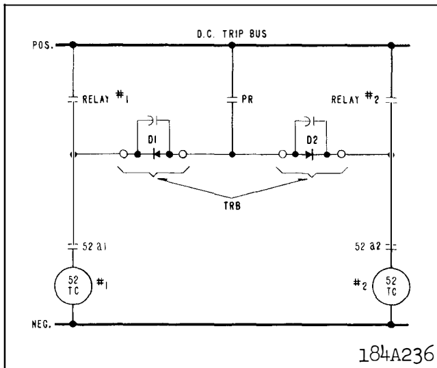
Fig. 2. Operational Schematic
