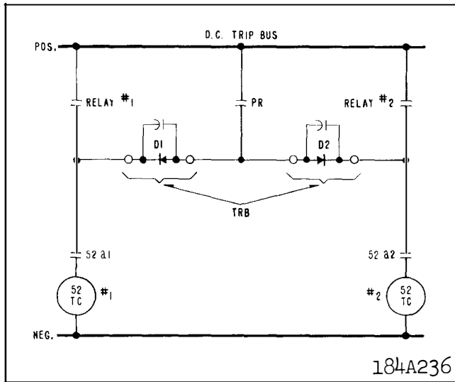
Fig. 2. Operational Schematic
