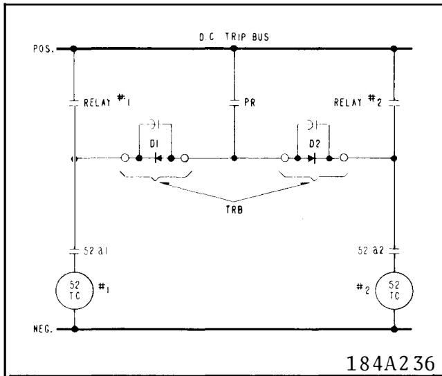
Fig. 2. Operational Schematic
