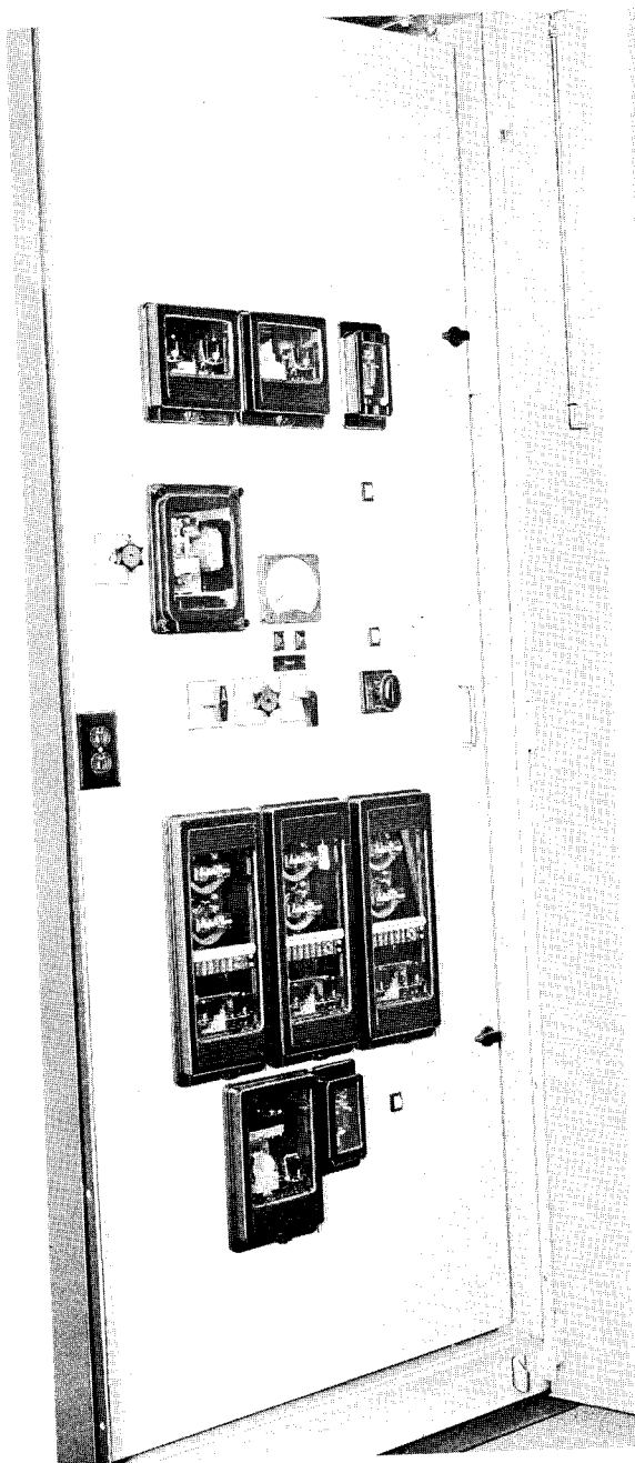
Fig. 15. Aisle-less: Standard Instrument Panel
