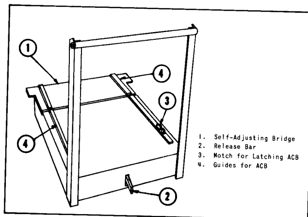
Fig. 36. Transport Truck
