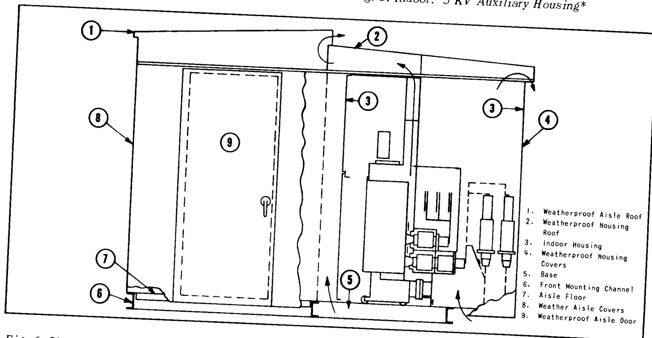
Fig. 6. Shelterfor-M: 5 KV Breaker Housing*
