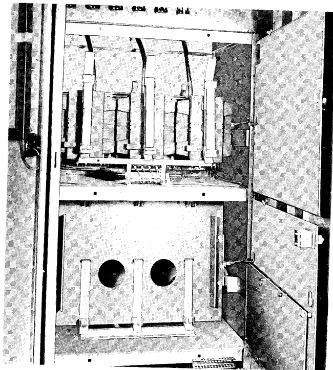
Fig. 26. Indoor and Outdoor: 15 KV Auxiliary Housing with PT and Fuse Doors Open
