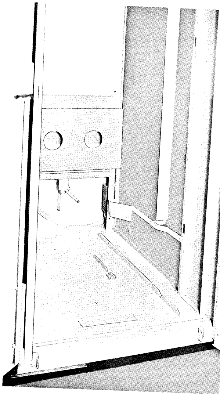
Fig. 13. Outdoor: F.V. Close-up showing Ventilating Screen and Transport Truck Clips
