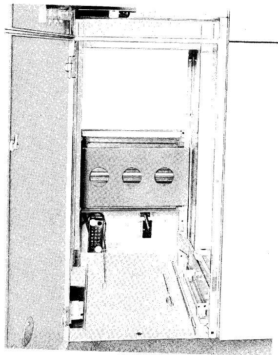
Fig. 18. Indoor and Outdoor: 5 KV Breaker Housing with Shutter and all Barriers in Place
