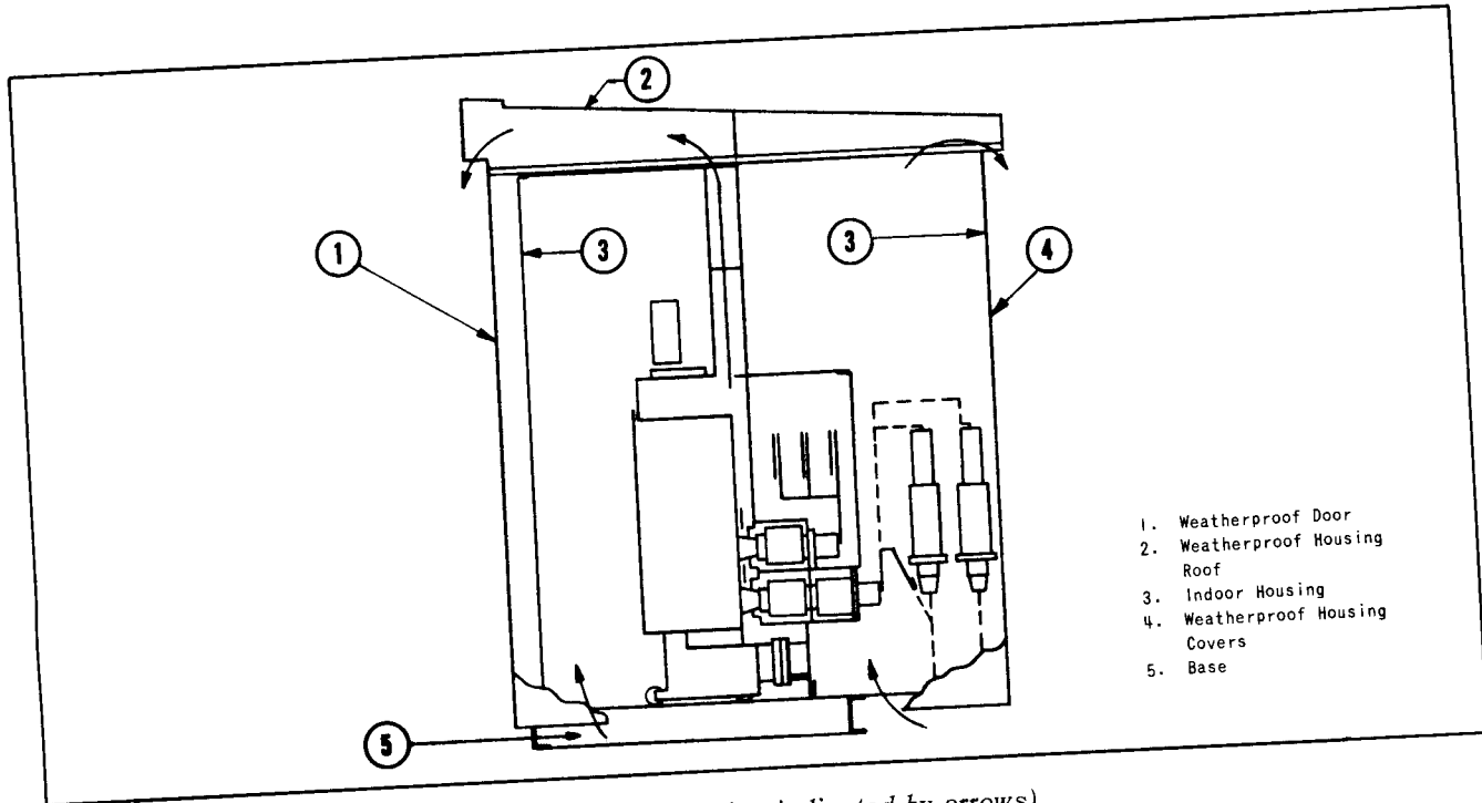
Fig. 7. Aisle-less: 5 KV Breaker Housing (Ventilation indicated by arrows)
