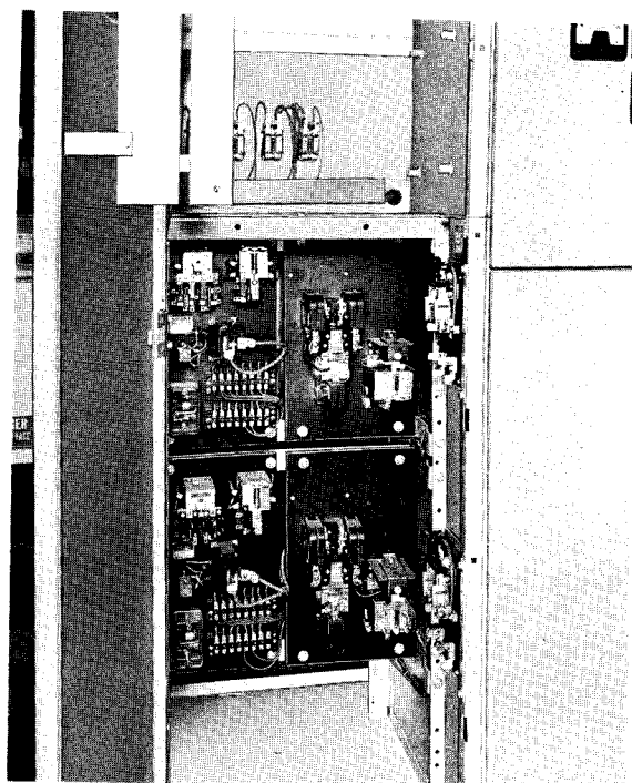
Fig. 28. Indoor and Outdoor: Field Control Equipment
