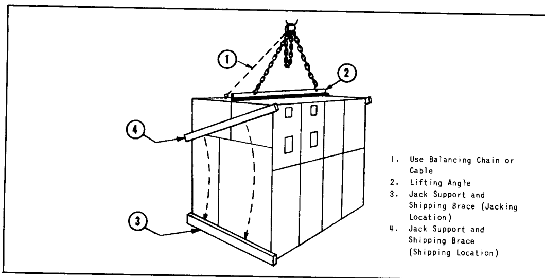
Fig. 39. Handling of Indoor Shipping Group
