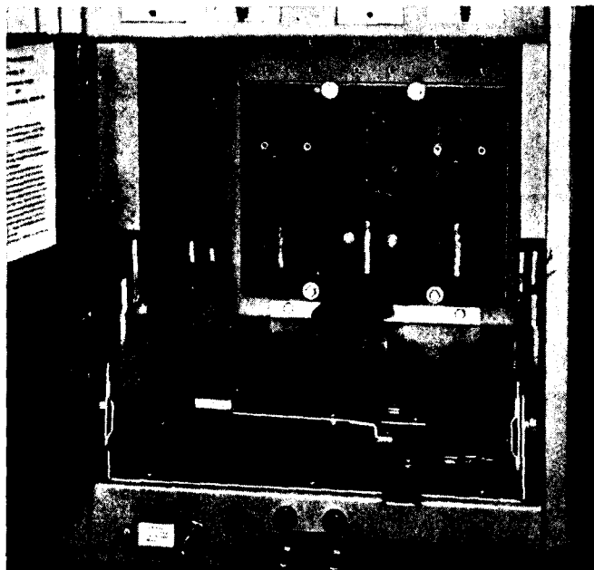
Figure 12: Insulating Boots
