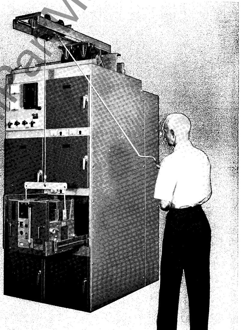
Figure 16: Traveling Lifter
