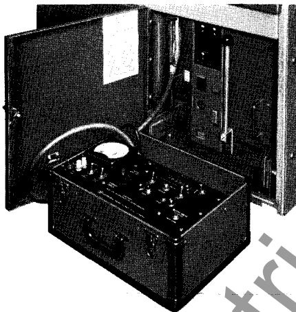
Figure 14: Test Kit
