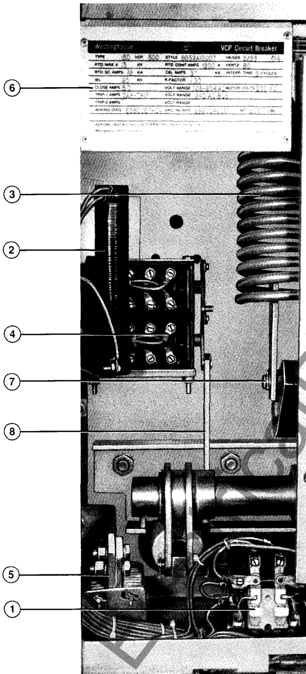
VAC-CLAD Switchgear Breaker Compartment
