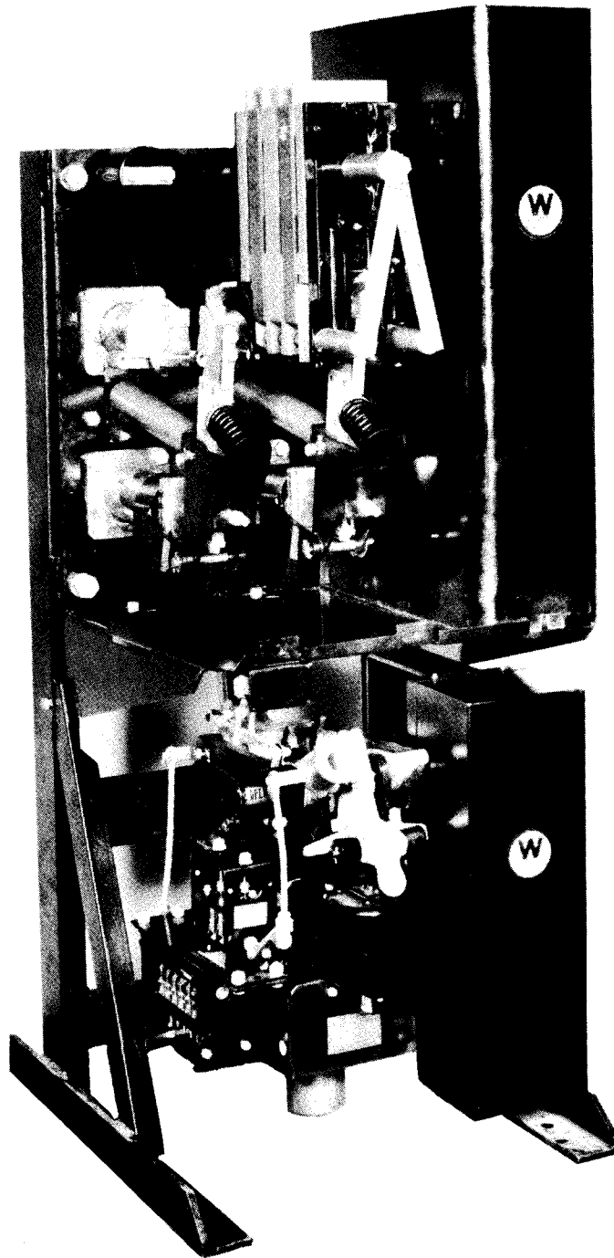
Figure 1 Type 50-U-20 "De-Ion" Air Circuit-Breaker Showing Pole Units in Various Stages of Assembly (Three-pole, 600-Ampere, 5000-Volt)
