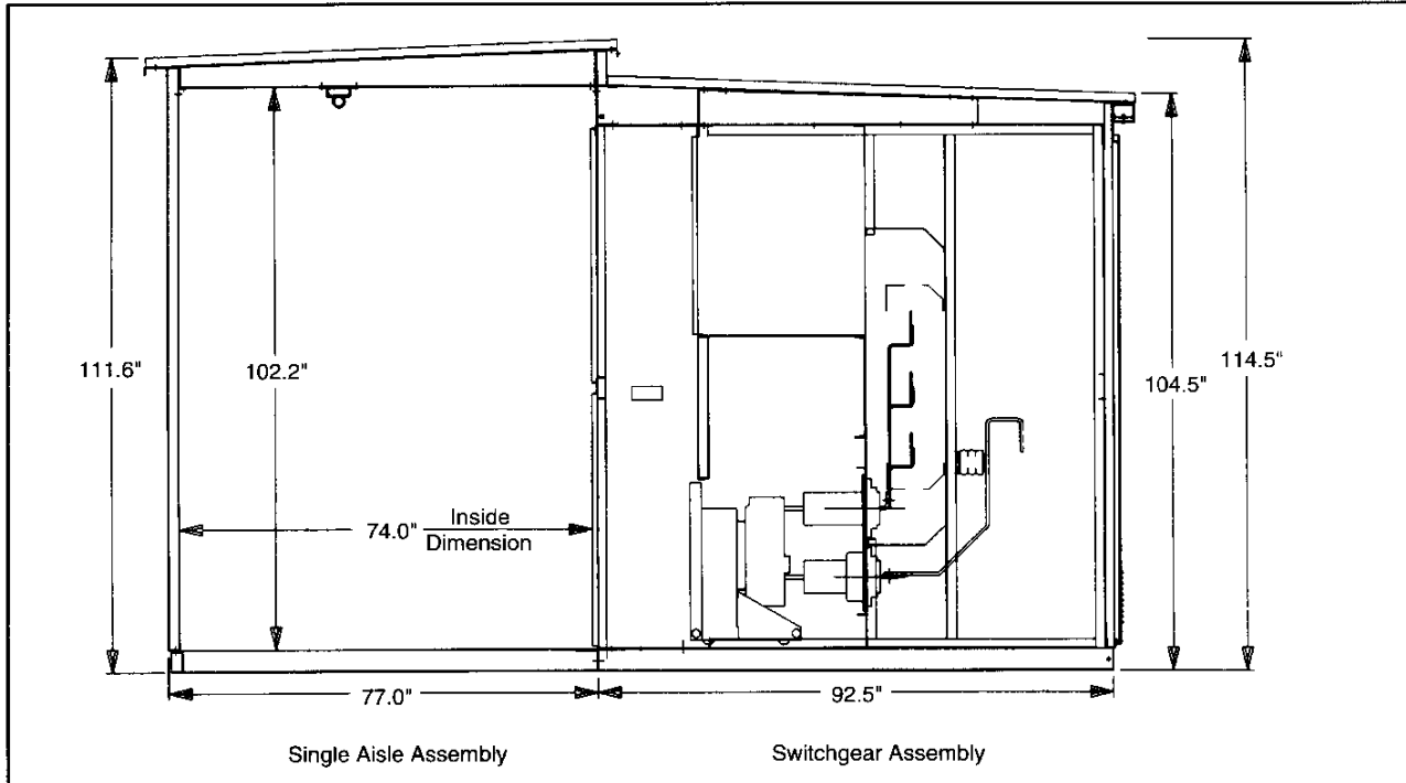
Single Aisle Enclosure
