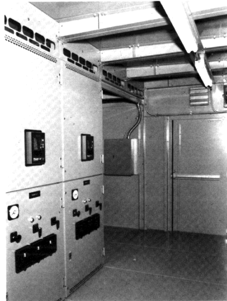
Front Aisle With Optional Work Area
