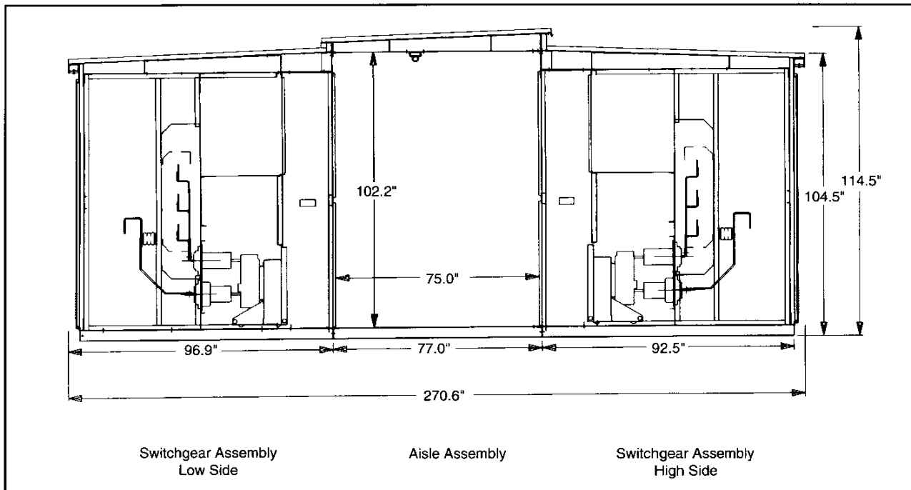
Common Aisle Enclosure With Double Row Switchgear
