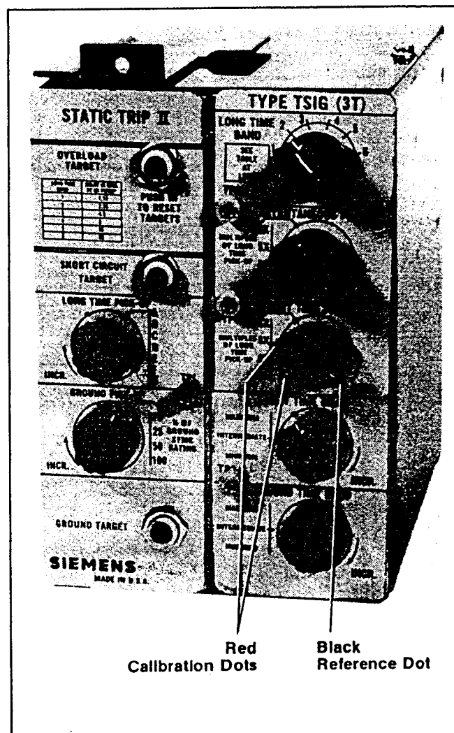
Figure 8. Calibration Marks
