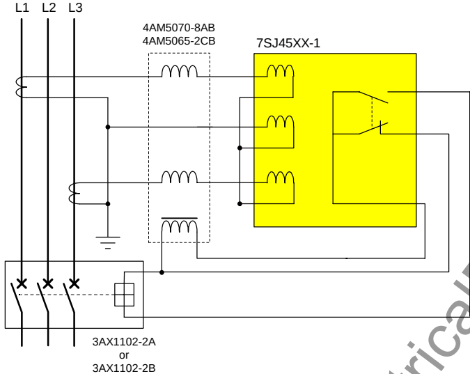
Figure 2-24 2-phase CT connection with auxiliary trip transformer and relay output
