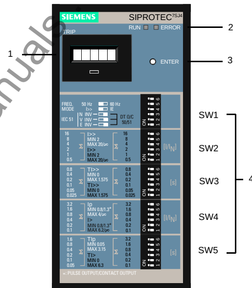
Figure 2-1 Device front with indication and control elements 7SJ45
