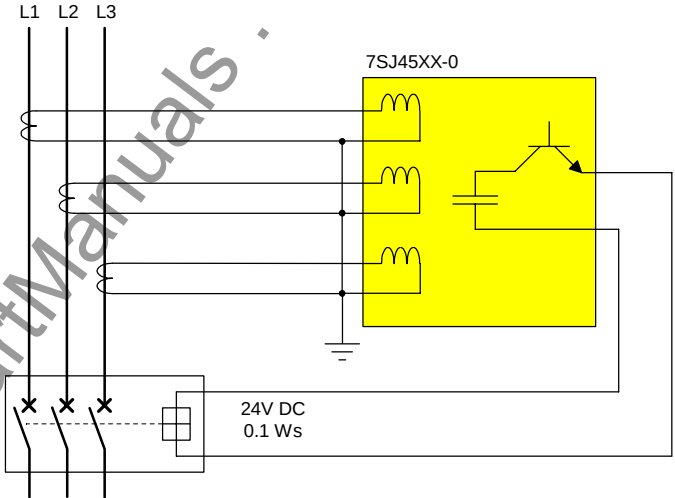
Figure 2-27 3-phase CT connection with pulse output
