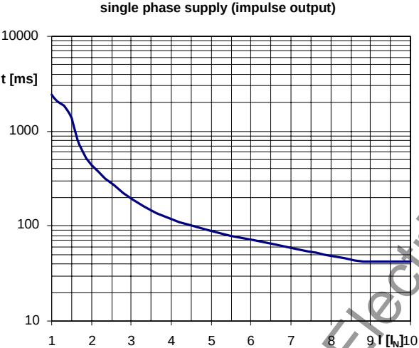
Figure 2-22 Maximum tripping time when switching onto a fault, device with pulse output
