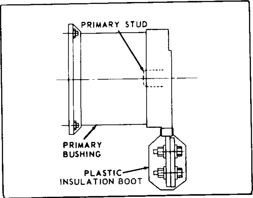
Figure 51. Installing Molded Plastic Boot - 15 kV
