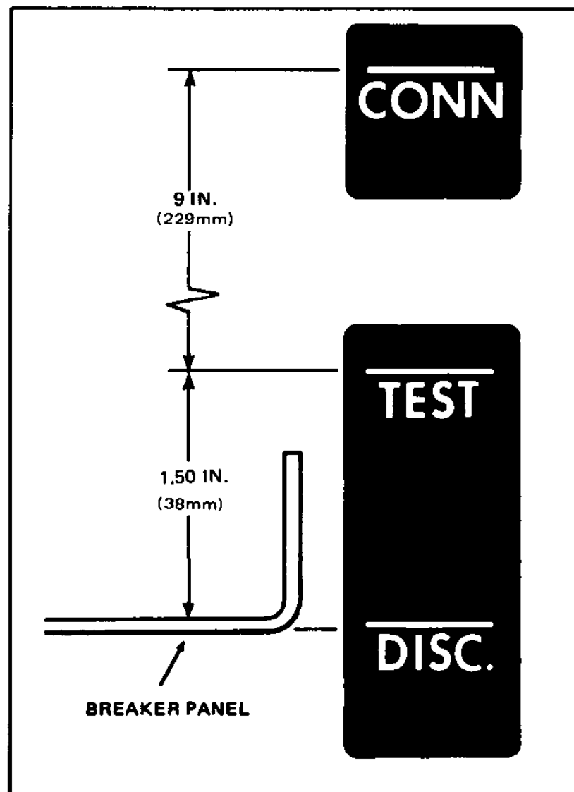
Figure 74. Circuit Breaker Position Indicator
