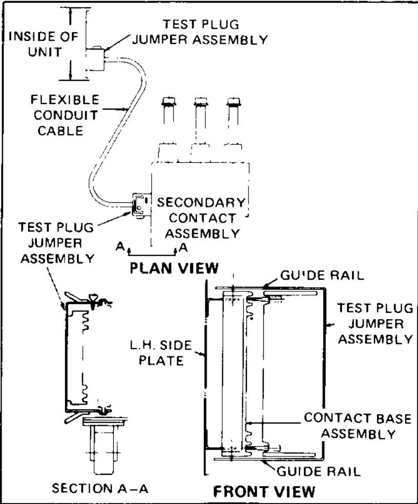
Figure 84. Connecting Breaker Secondary to Cubicle.
