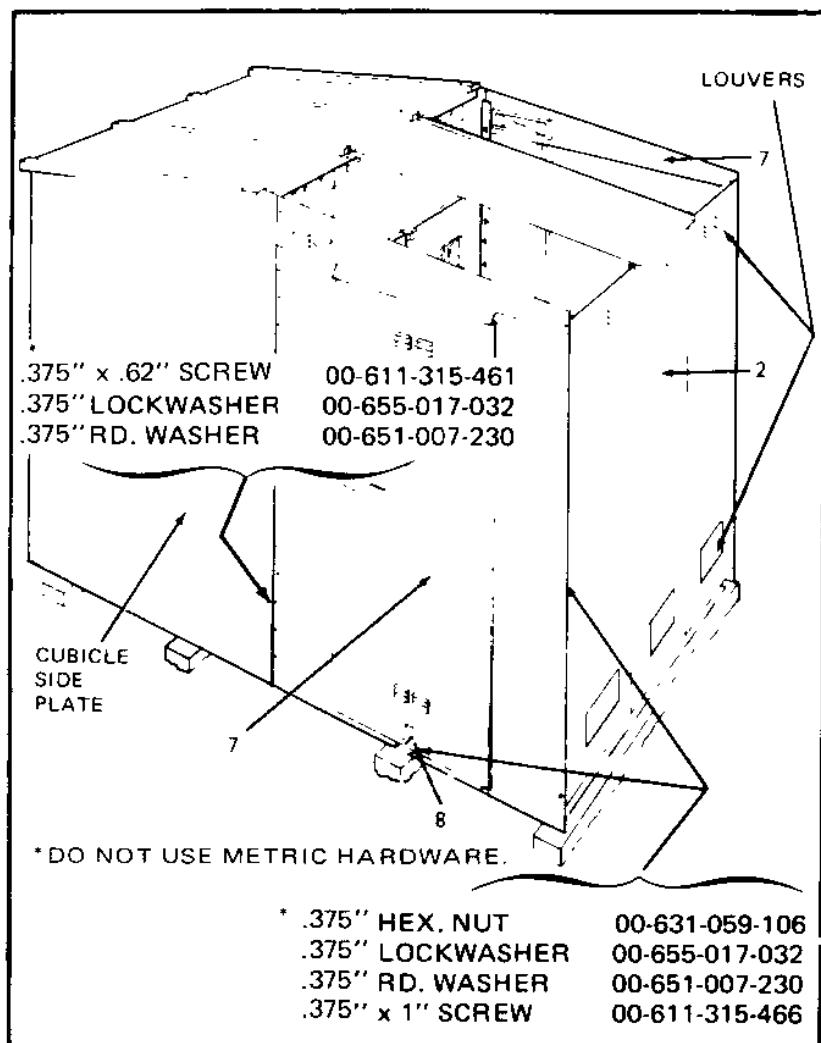
Figure 27. Door Installation – Single Aisle Layout
