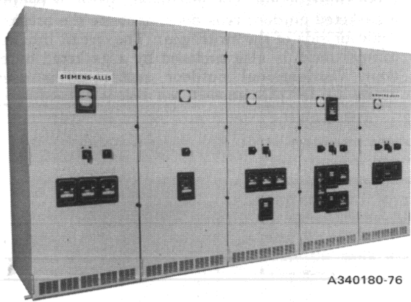
Figure 2. 15 KV Indoor Switchgear Installation
