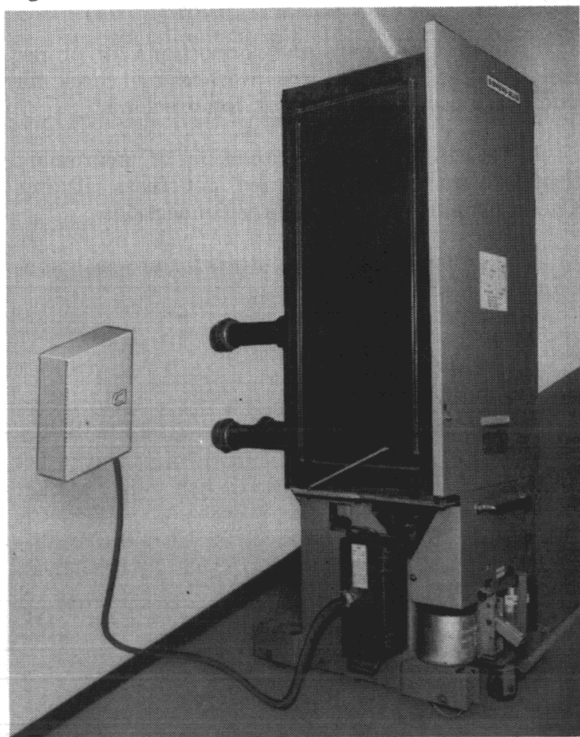
Figure 82. Testing Breaker Outside Unit with Test Cabinet.
