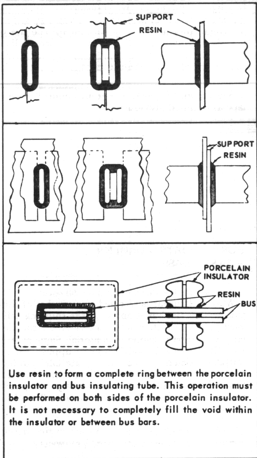
Figure 54. Caulking Bus Supports
