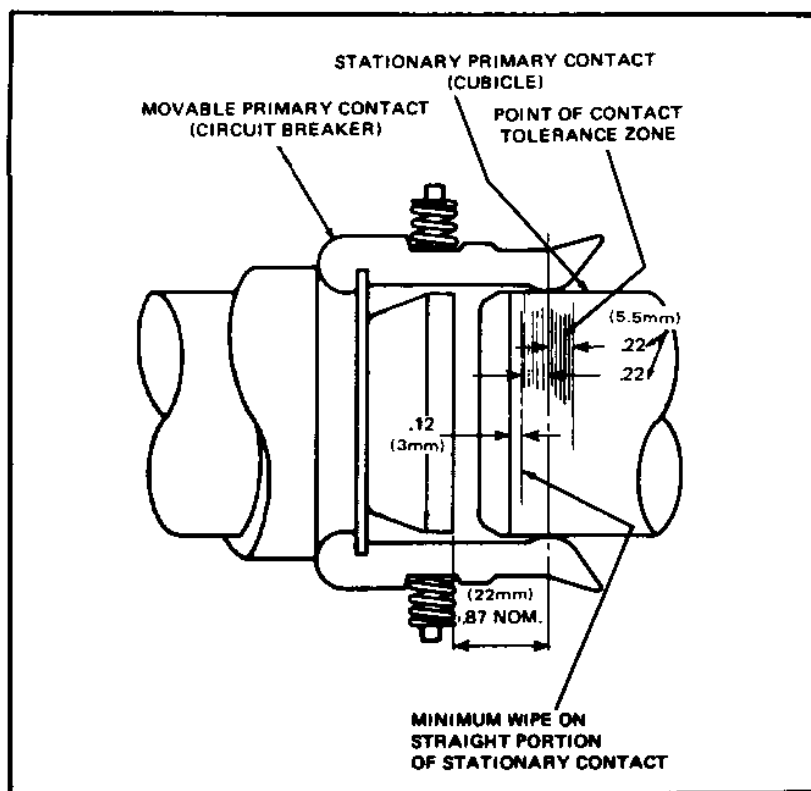
Figure 75. Primary Contact Engagement.
