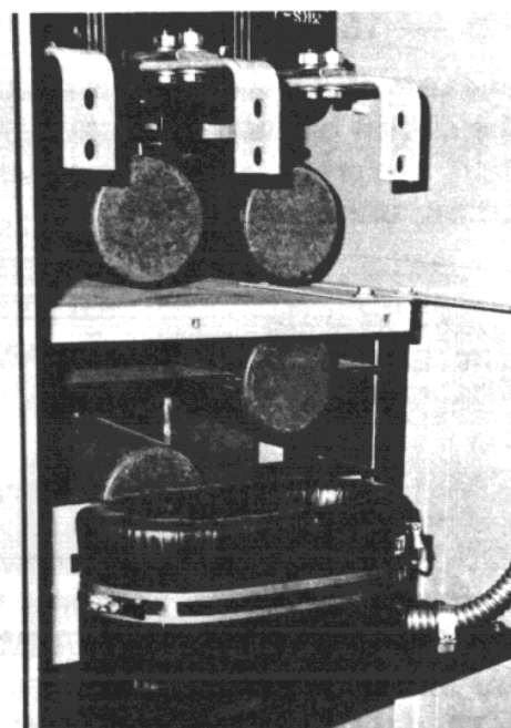
Figure 71. Elliptical Torroidal Current Transformer (Ground Sensor)
