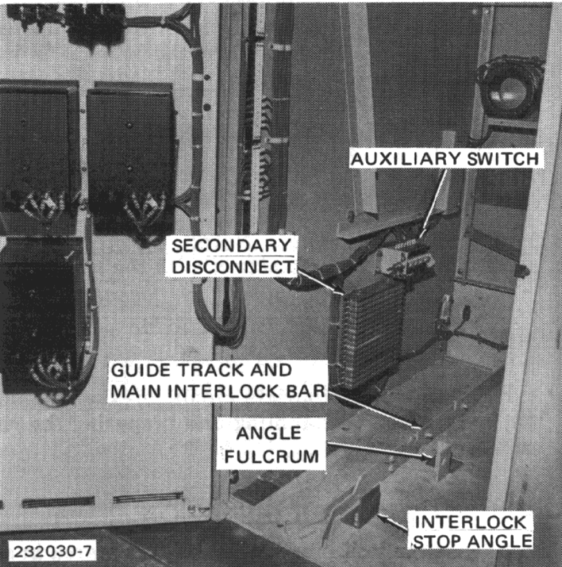
Figure 72. Positioning Interlocking and Operating Devices
