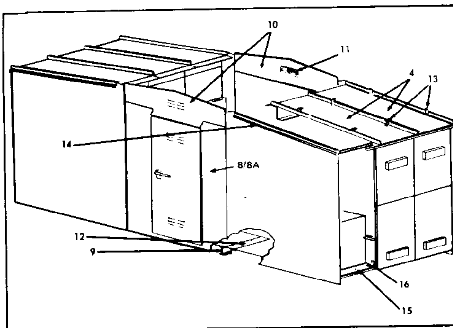
Figure 45. Installing New Equipment
