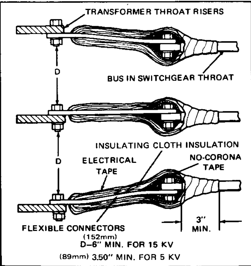
Figure 53. Insulating Transformer-to-Bus Bar Joints
