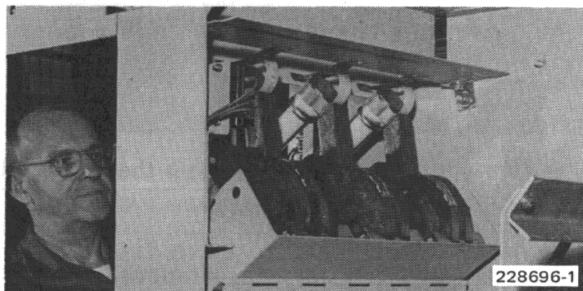
ROTATE BASE 135°, FUSES GROUNDED
