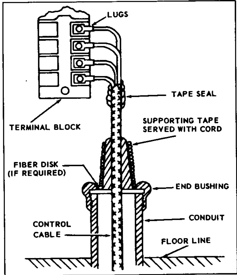
Figure 64. Secondary Control Cable Connections
