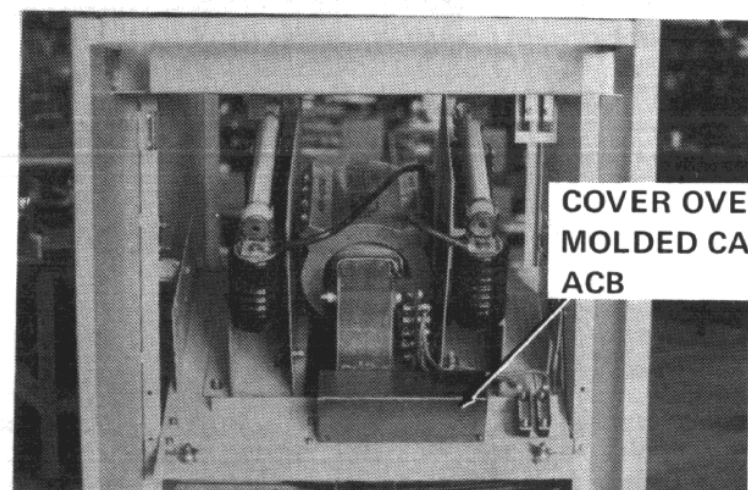
Figure 67. Location and Mounting of Current Transformers
