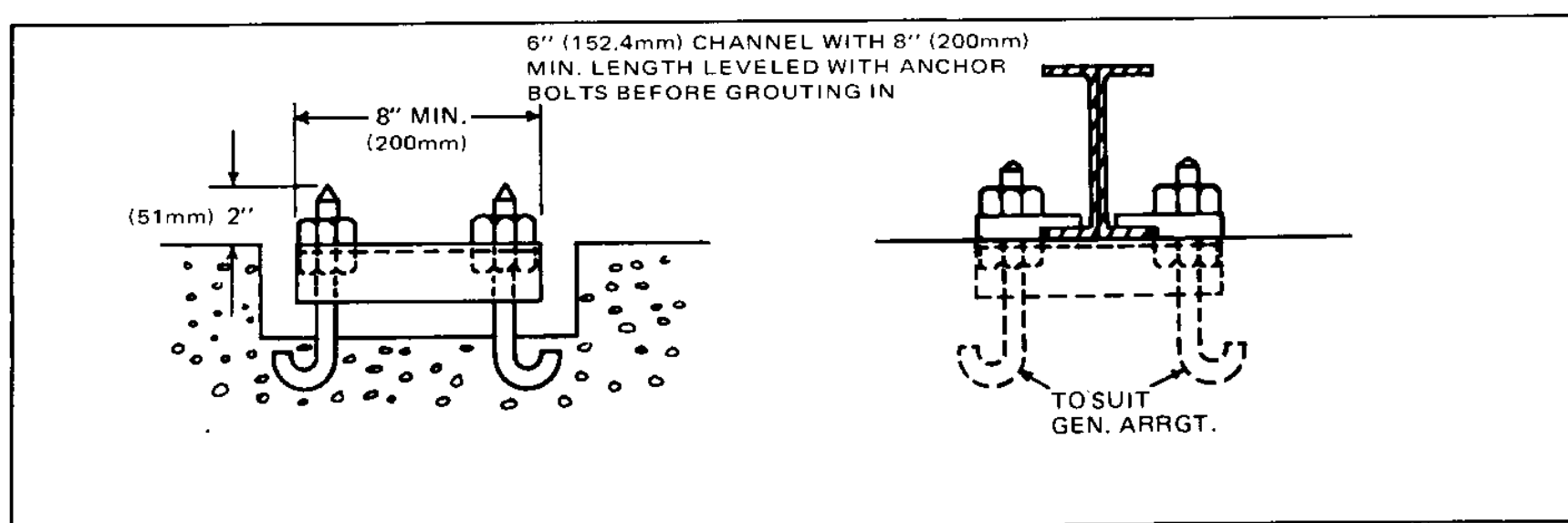
Figure 13. Securing Outdoor Cubicles
