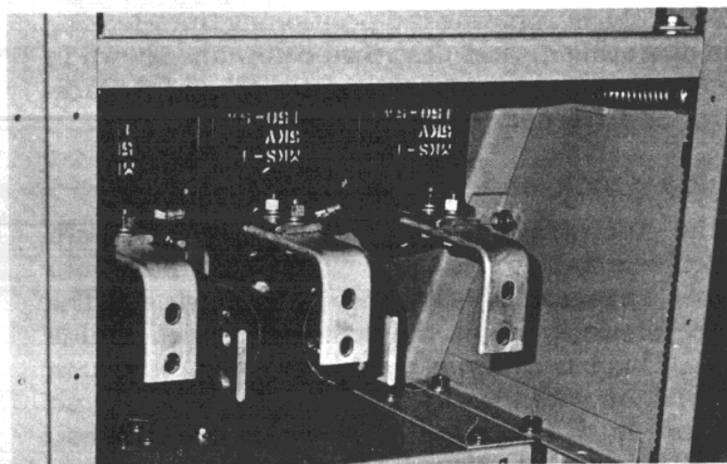
Figure 69. Wound or Bar Type Current Transformers
