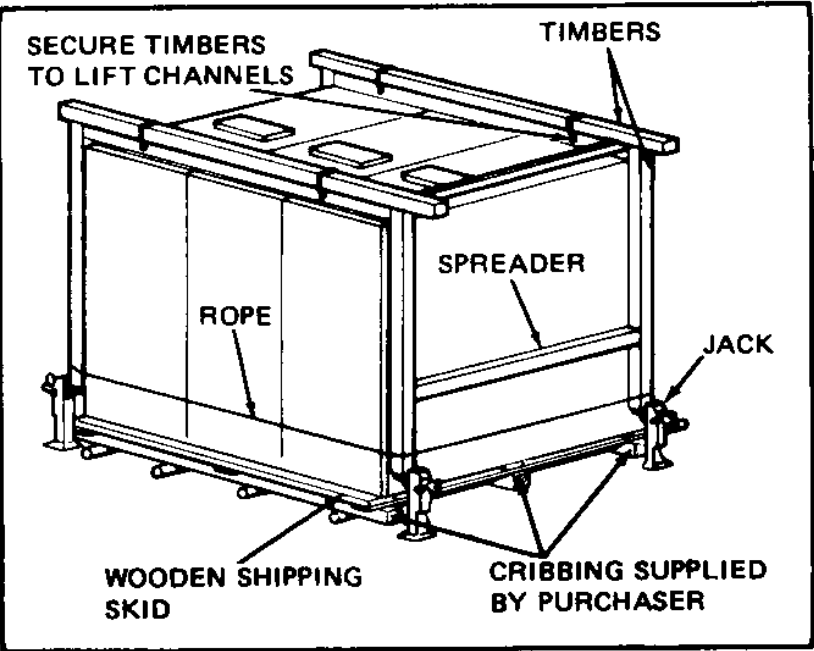
Figure 9. Jacking Indoor Switchgear
