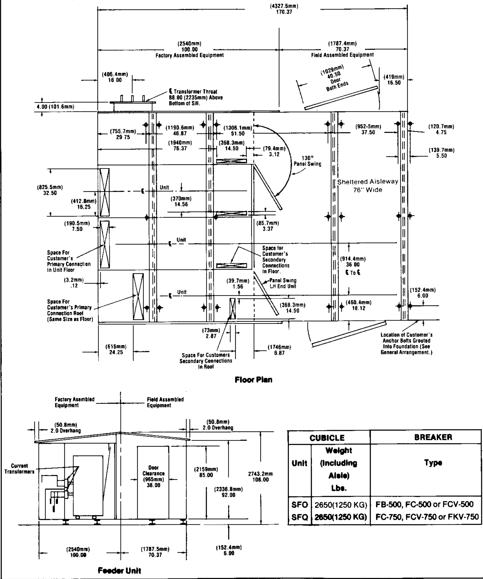
Figure 19A. Floor Plan and Typical Side View of 15 kV Low Silhouette Single Aisle Shelter-Clad Cubicles
