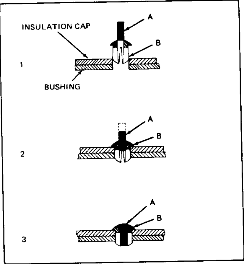
Figure 50. Inserting Nylon Rivet – 5 kV
