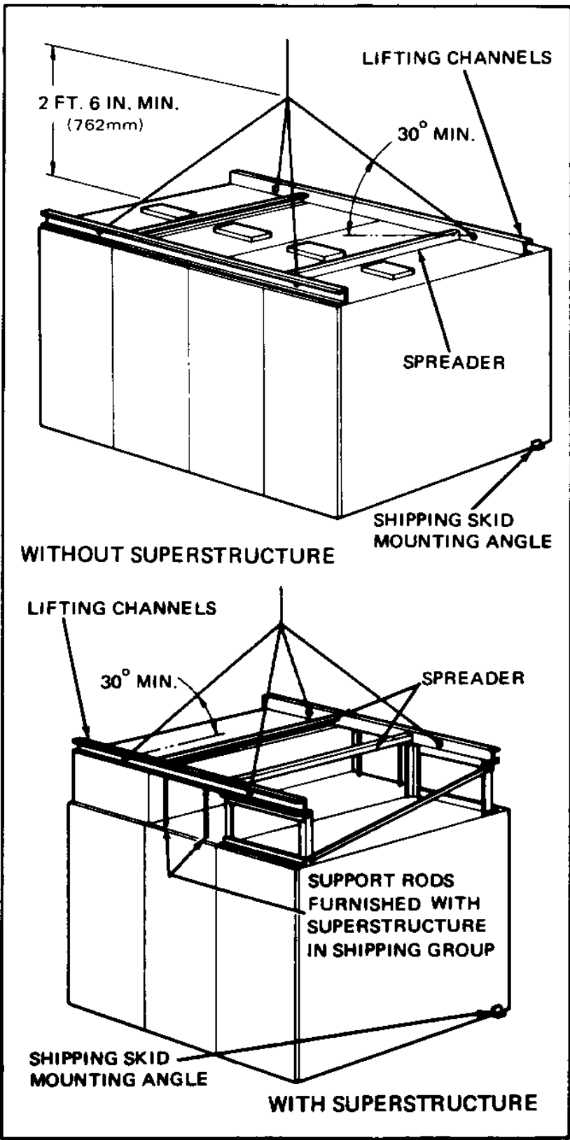
Figure 6. Lifting 15 kV Indoor Switchgear
