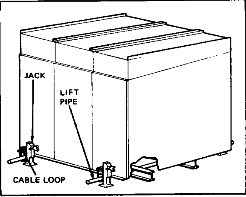
Figure 10. Jacking Shelter-Clad and 5 kV Conventional Outdoor Switchgear
