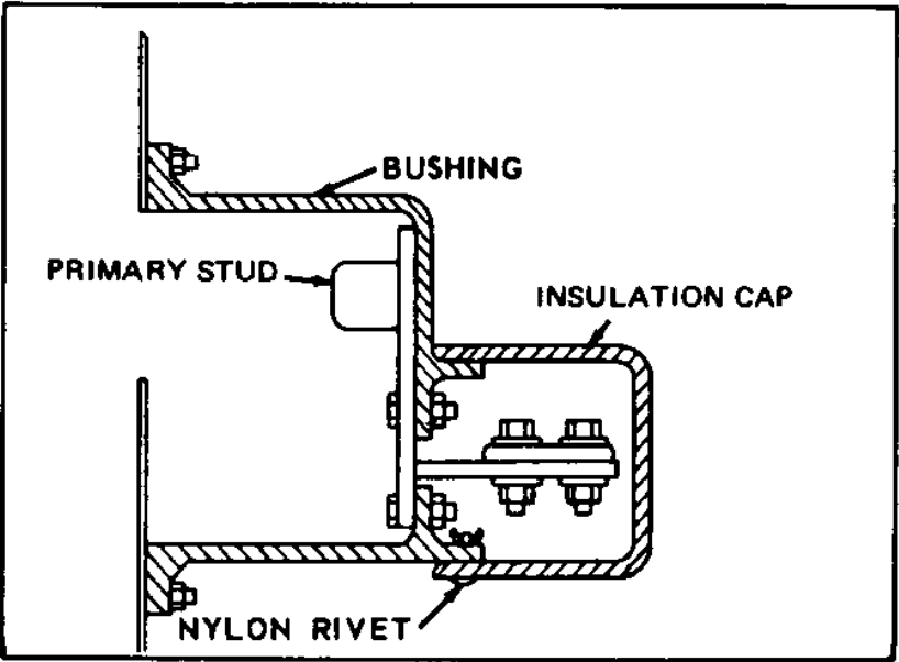
Figure 49. Insulation Cap Installation – 5 kV Bus Joints
