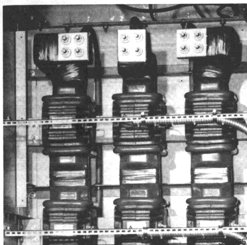
Figure 70. Bar-Type Current Transformer Application
