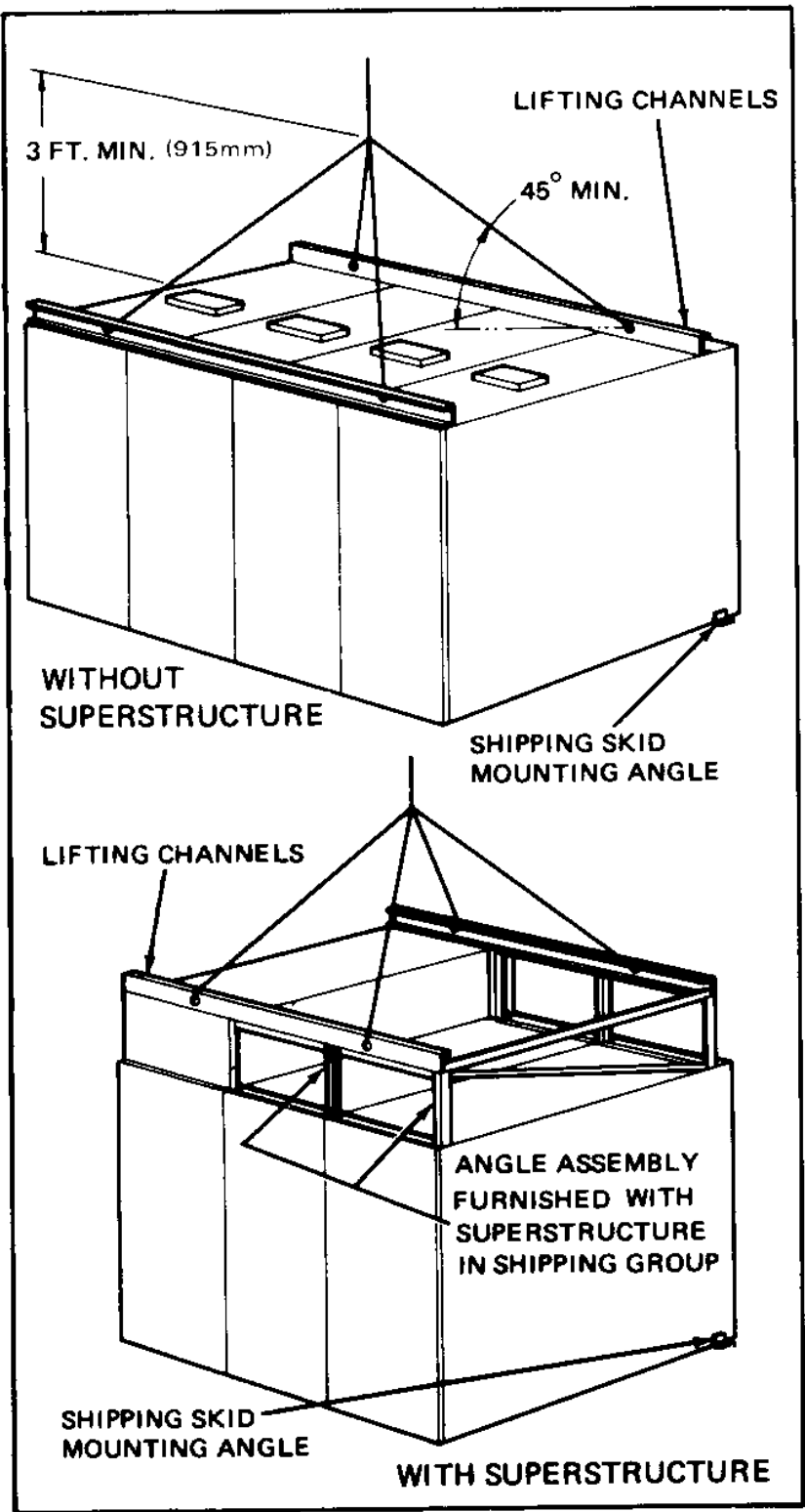
Figure 5. Lifting 5 kV Indoor Switchgear
