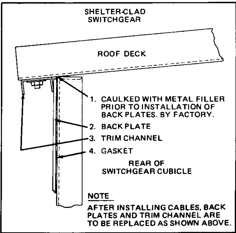
Figure 61A. Back Plate Mounting After Cable Installation
