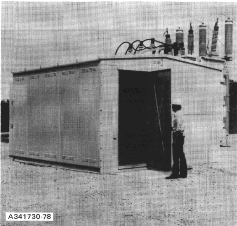
Figure 4. 5 kV Conventional Outdoor Switchgear
