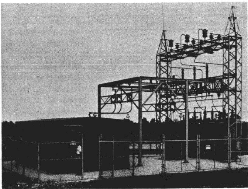
Figure 3. 15 KV Shelter-Clad Switchgear Installation
