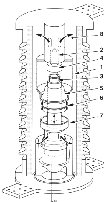
Breaking chamber
