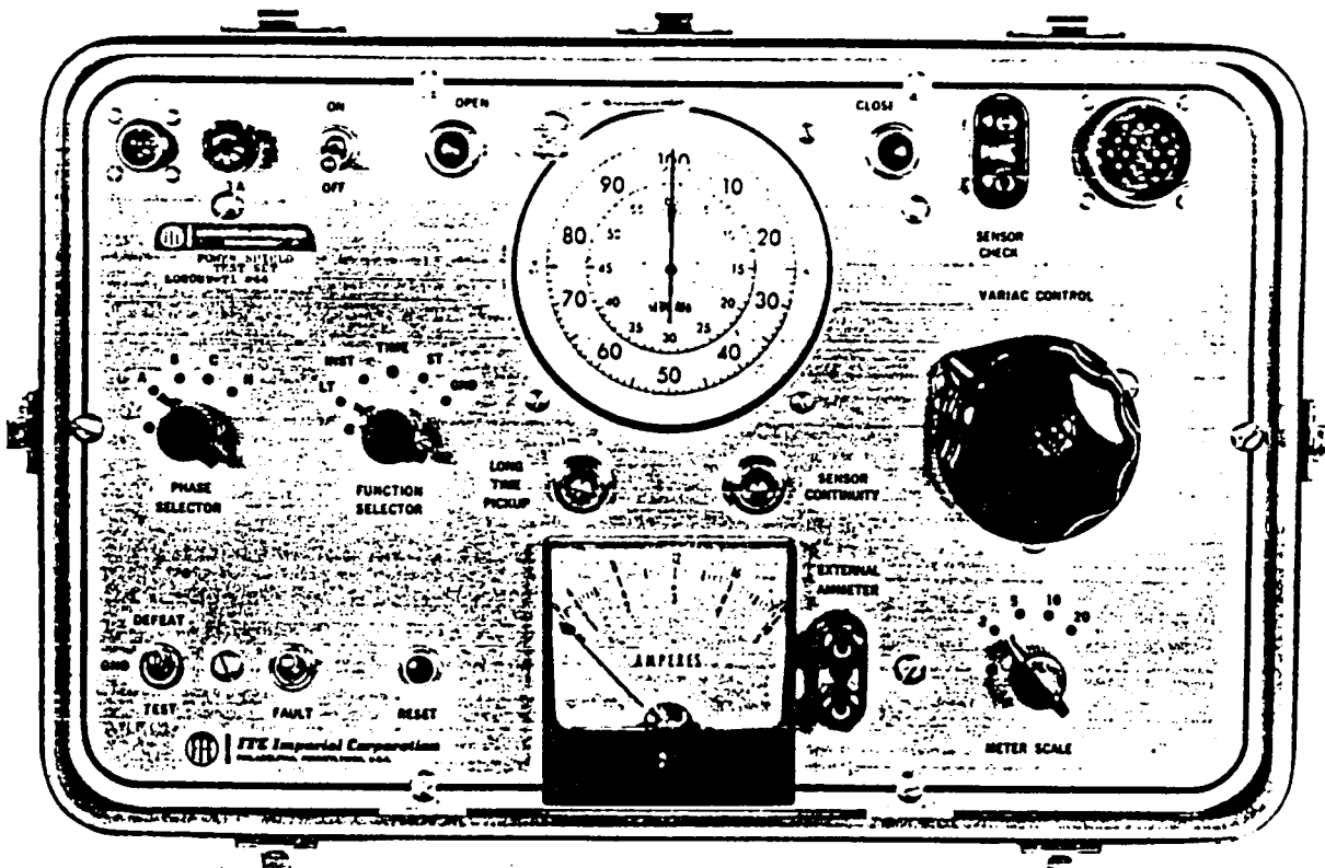
Front View of Test Set Showing Location of Controls
