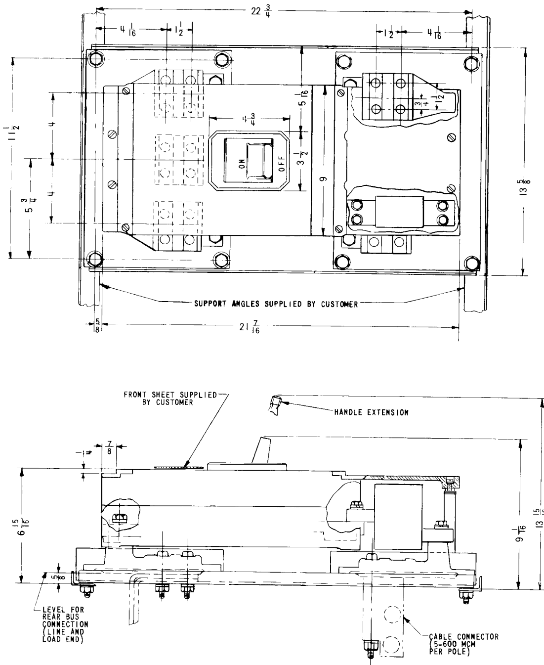
Fig. 9 — 2000-Ampere CR-Frame Circuit Breaker Dimensional Drawings with Reverse Mounting Block Assembly
