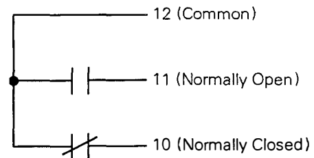
Figure 2. Bell Alarm with Lockout connections on the right terminal block, with contacts shown in the reset state.
