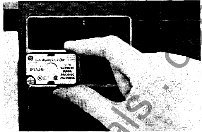
Figure 4. Inserting the Bell Alarm with Lockout into the accessory compartment.
