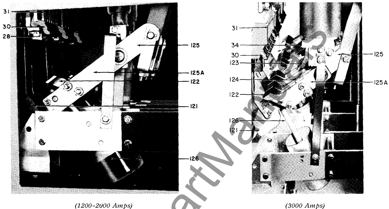
Fig. 4. Contact assembly (Ref. No. 120)
