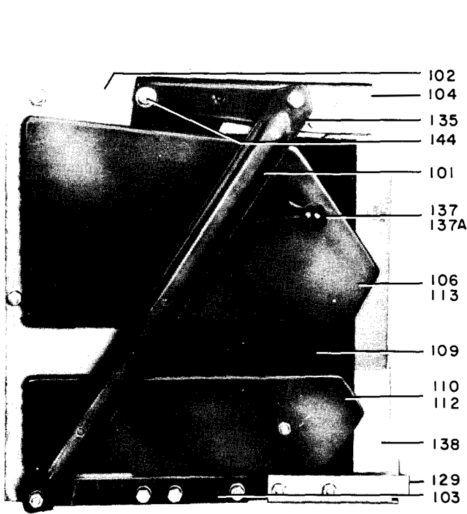
A. Complete arc chute assembly "-6" design
