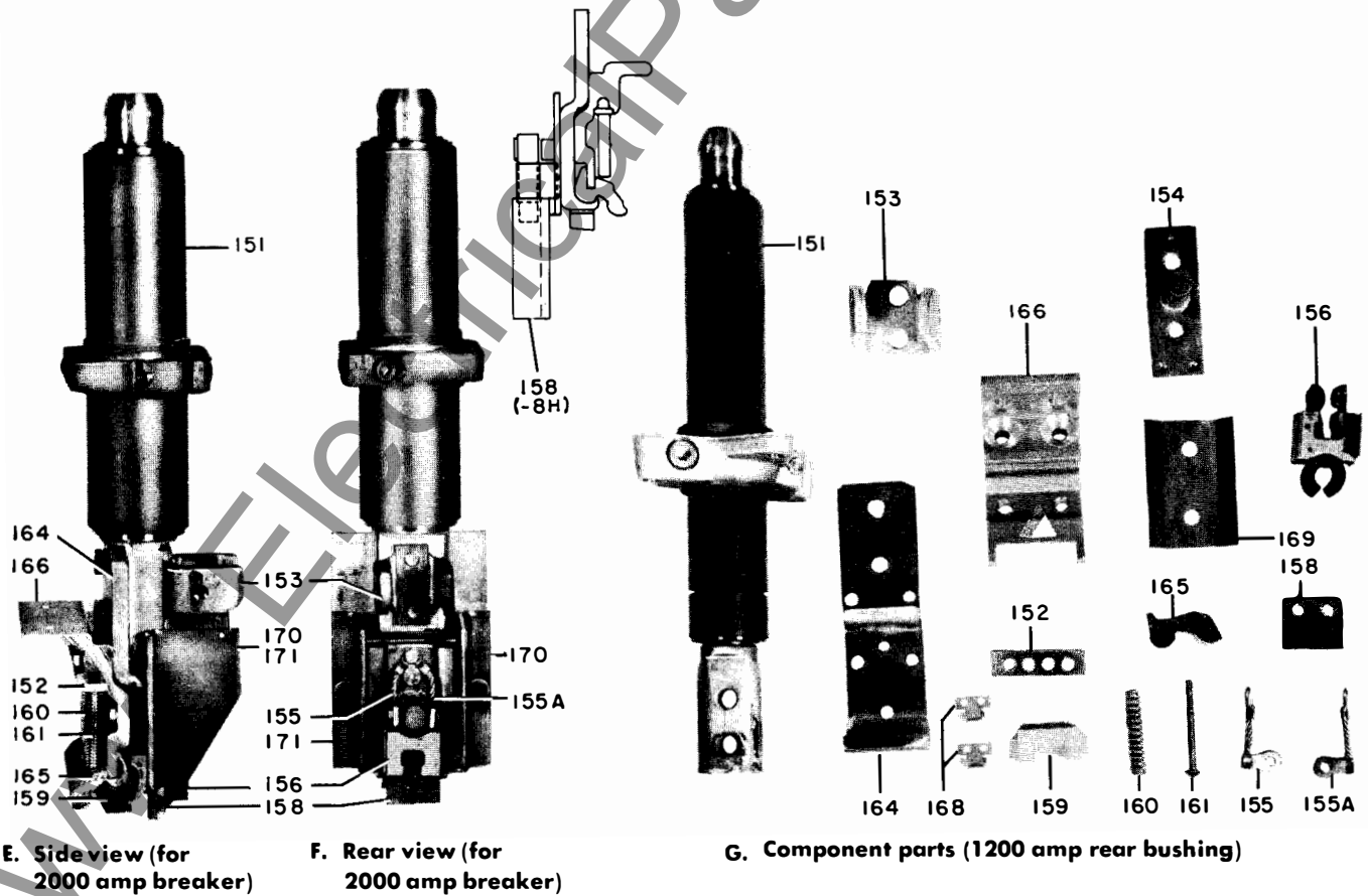
Fig. 3. Rear bushing assembly (Ref. No. 150)
