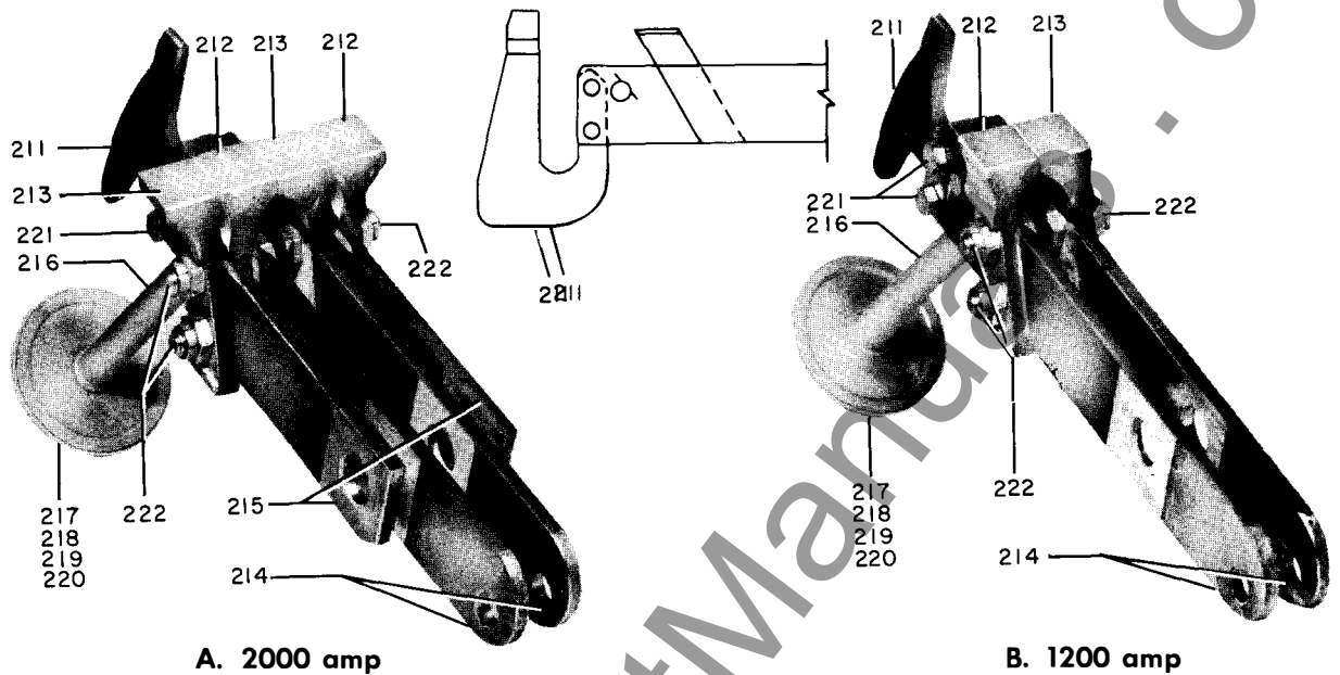
Fig. 4. Movable contact arm assembly (Ref. No. 210)
