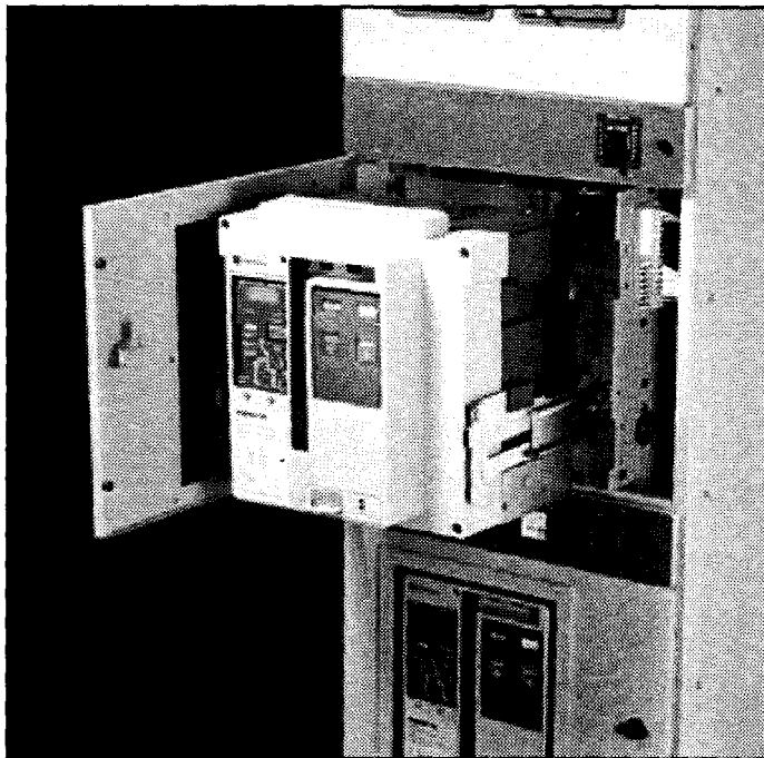
Figure 3-3 Magnum DS Breaker on Extension Rails
