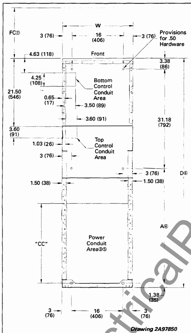
Drawing 2A97850
