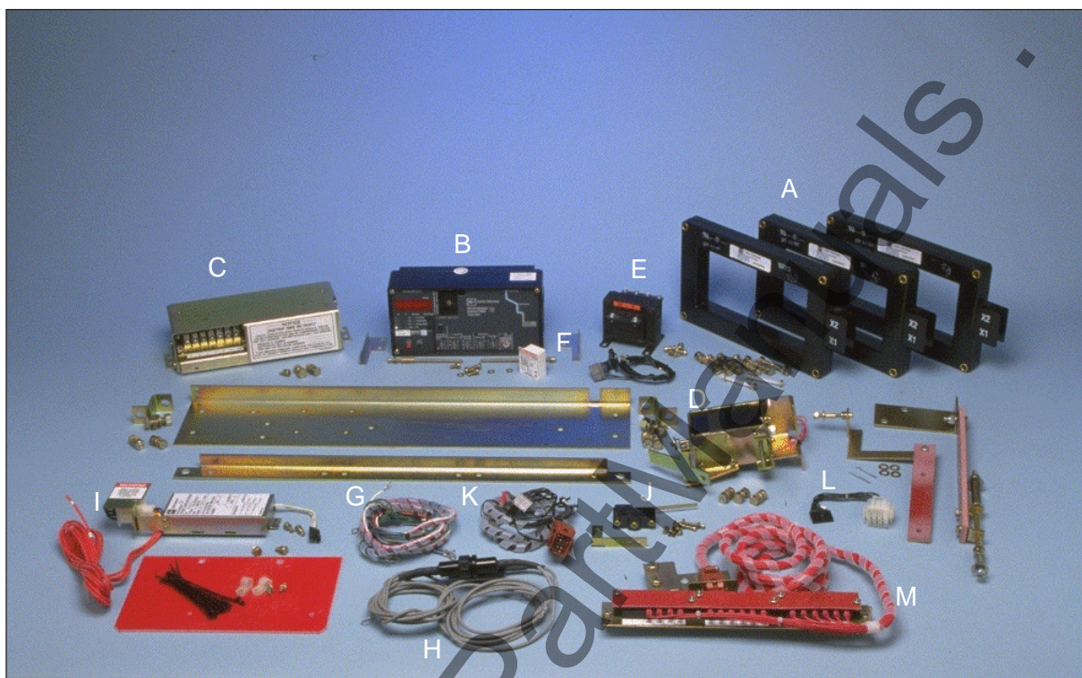
Fig. 36 Retrofit Components
