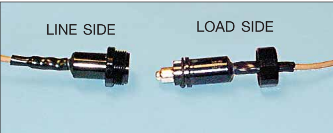
Fig. 15 Identification of the Line and Load Side HV Wires.
