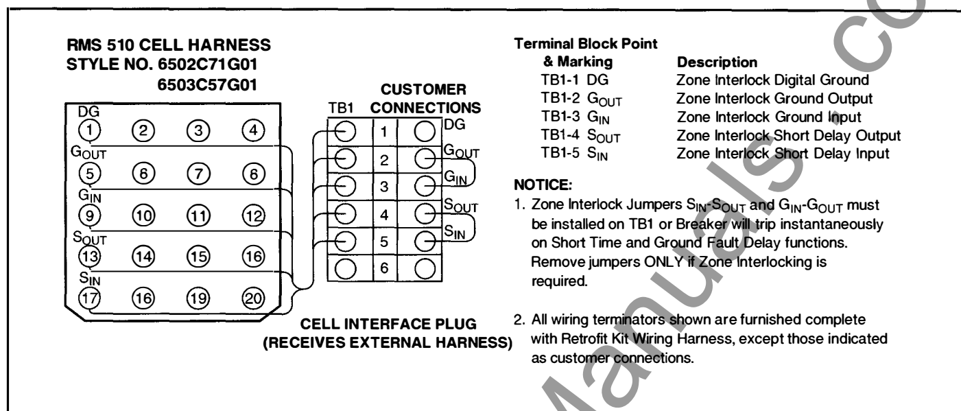
Fig. 12-12 Digitrip RMS 510 Cell Harness
