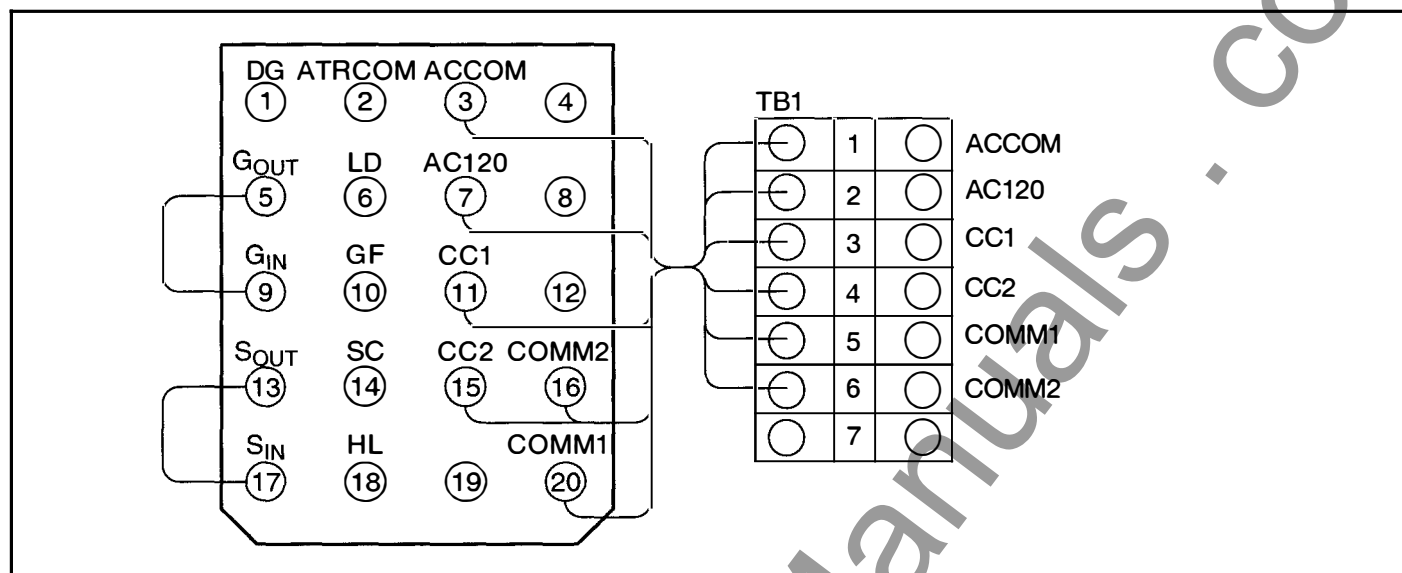
Fig. 12-15 Digitrip RMS 810 &amp; 910 Simplified Cell Harness
