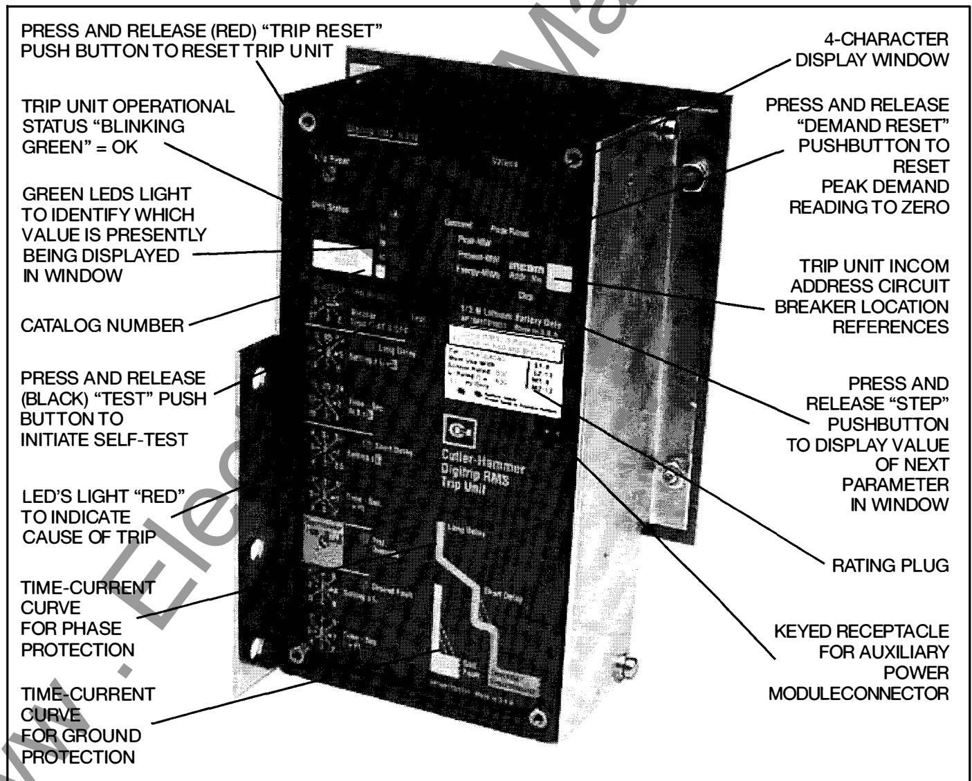
Fig. 10-4 Digitrip Trip Unit Display Panel
