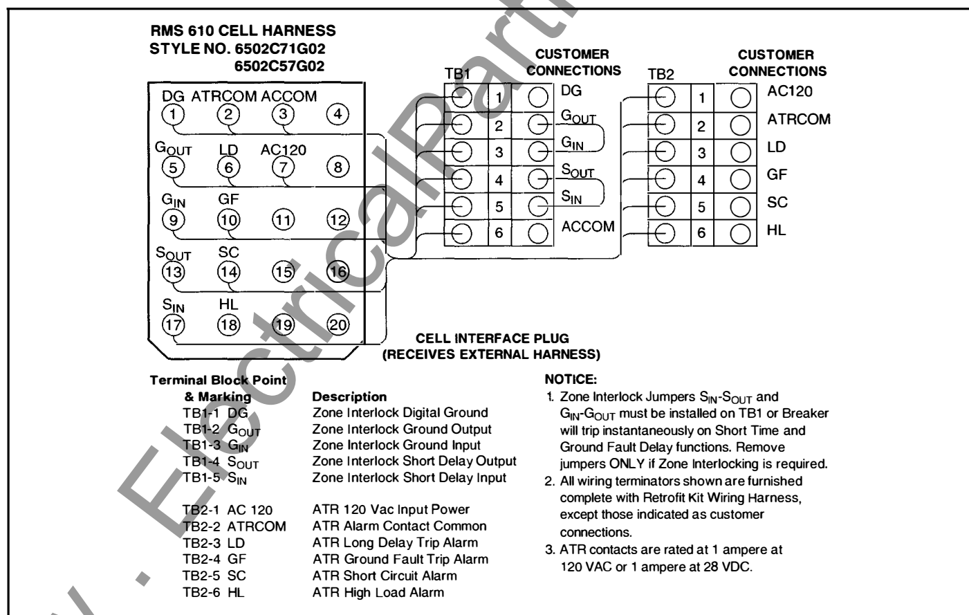
Fig. 12-13 Digitrip RMS 610 Cell Harness
