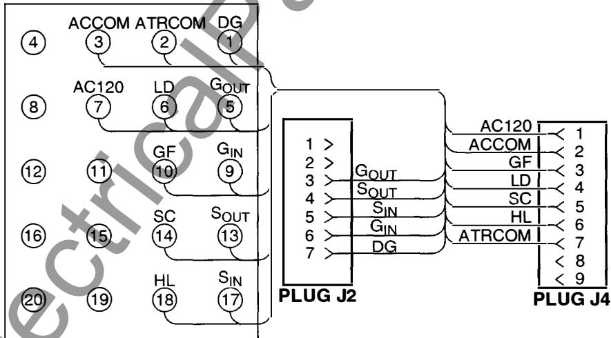
Fig. 12-9 Digitrip RMS 610 External Harness
