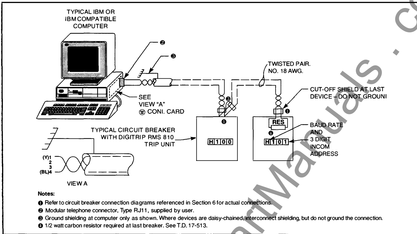
Fig. 10-5 Terminating Resistor Location
