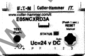
Overload Relay with Cover Closed (front view)
