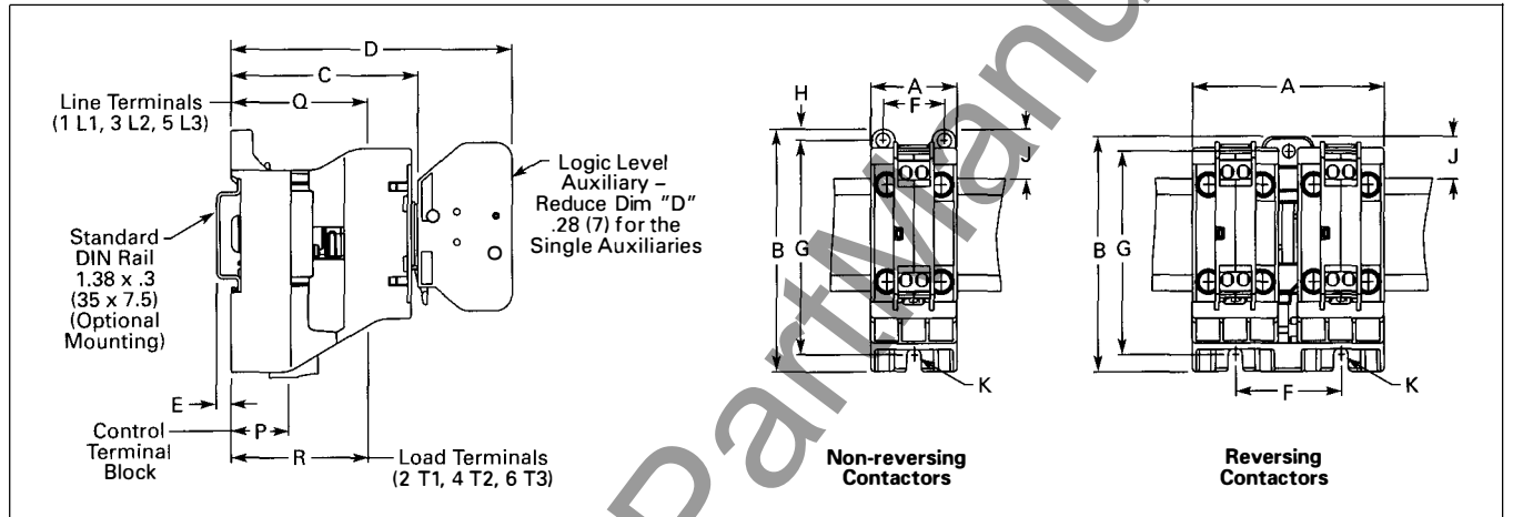
Figure 34-6. Approximate Dimensions — Inches (mm)
