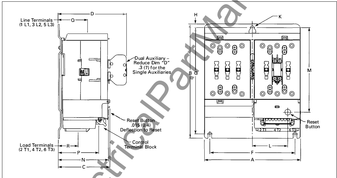
Figure 34-11. Approximate Dimensions — Inches (mm)
