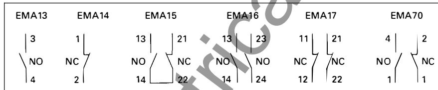
Figure 34-5. Connecting Diagram — A – E Frames
