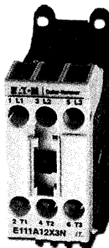
IEC A-Frame FVNR Contactor Cat. No. E111A12X3N
