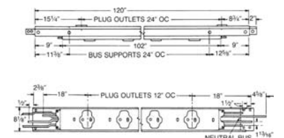
Standard lengths, three-phase, four-wire systems, 480 Y/277 Volts
