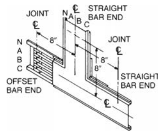
Tee Up
