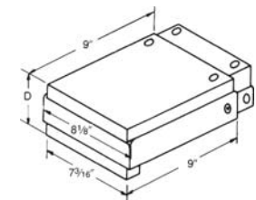
End box used to close off end-of-run.
