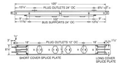
Standard lengths, three-wire systems, 600 volts maximum.
