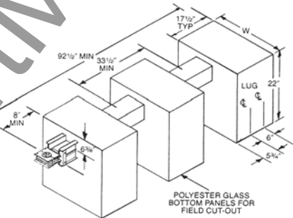
Single-Phase Transformer Taps
